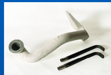
Parts for fibre guiding
